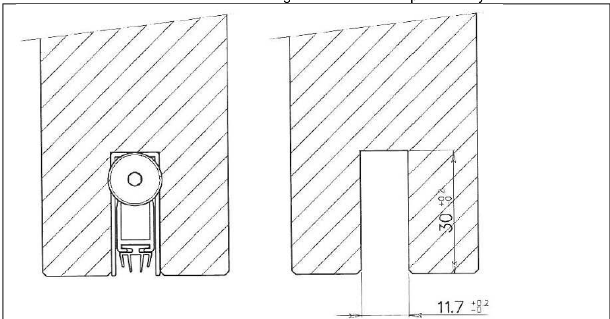
Figure 1 Sectional drawing 11.7/30 ASGSFI-A
