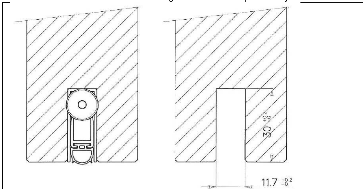
Figure 1 Sectional drawing 11.7/30 ASGSFI-B
