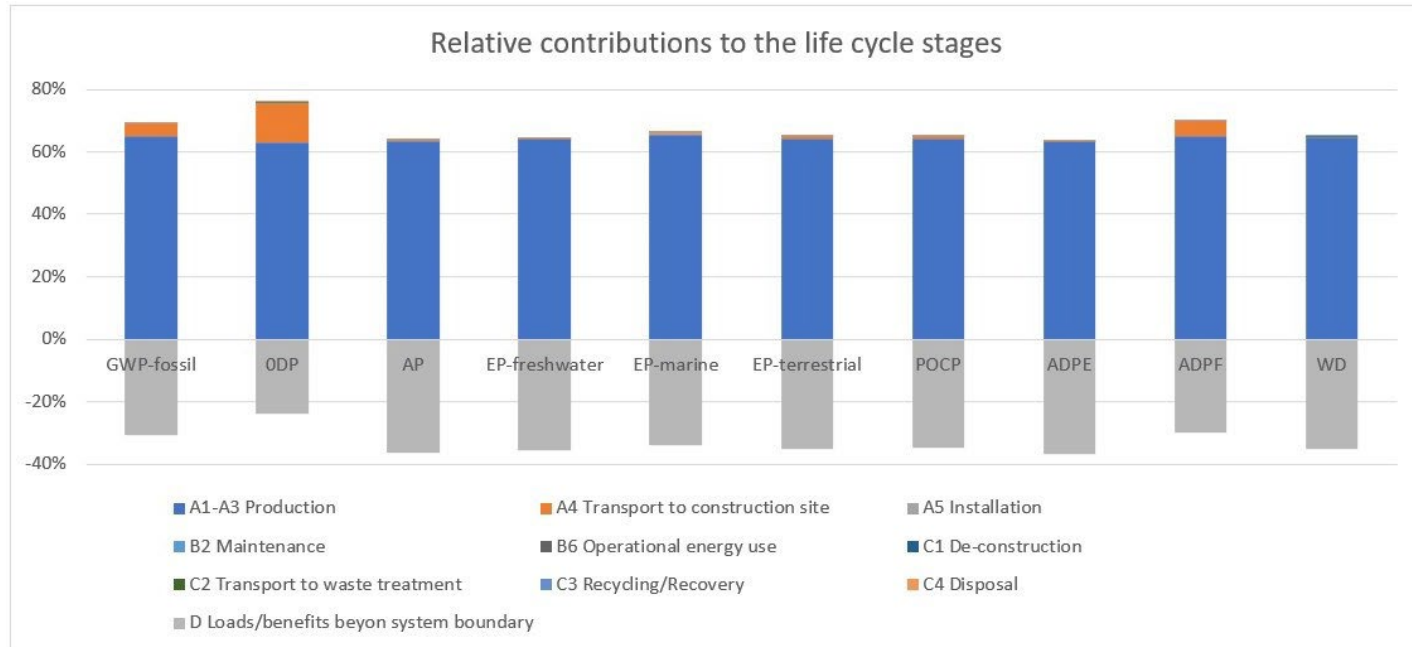
Figure 1: Environmental impacts of lock cyclinders along its life cycle
