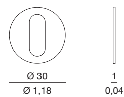
C. BOCCHETTA TONDA SLIM FORO CHIAVE DIAMETRO 30 MM - 1,18 INCH ROUND SLIM KEY HOLE ESCUTCHEON DIAMETER 30 MM - 1,18 INCH
