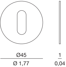
D. BOCCHETTA TONDA SLIM FORO CHIAVE DIAMETRO 45 MM - 1,77 INCH ROUND SLIM KEY HOLE ESCUTCHEON DIAMETER 45 MM - 1,77 INCH
