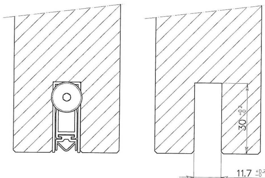
Figure 1 Sectional drawing 11.7/30 ASGSFI-CO
